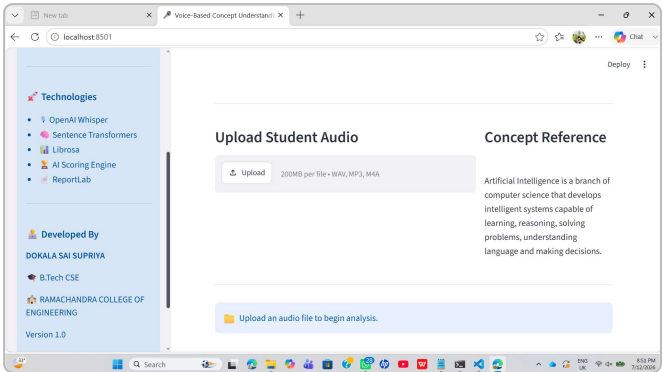
Figure 5: Home Page
