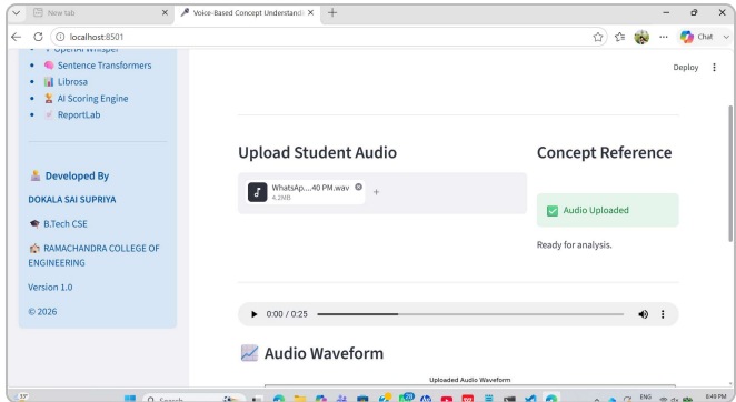
Figure 6: Audio Upload
