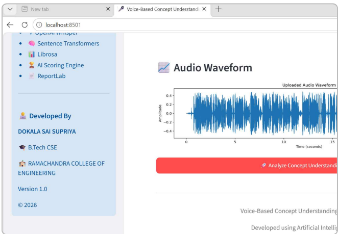
Figure 7: Audio Waveform
